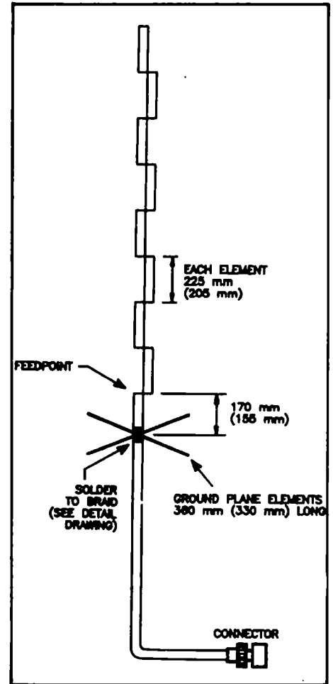
Figure 3. The general form of the UHF coaxial collinear antenna described. Dimensions are shown for the 70cm amateur band and the UHF CB band (in brackets).
