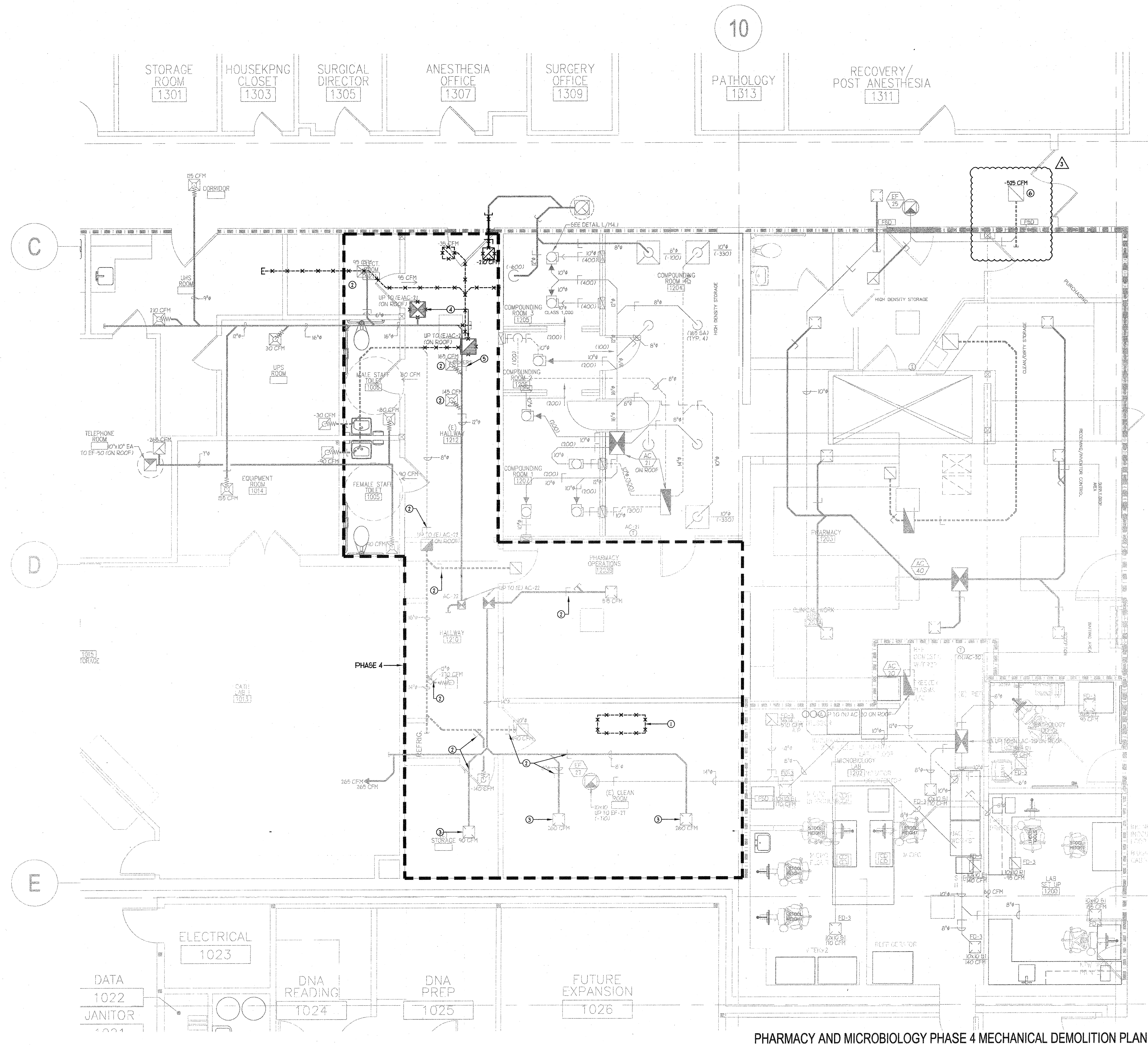
PHARMACY AND MICROBIOLOGY PHASE 4 MECHANICAL DEMOLITION PLAN
