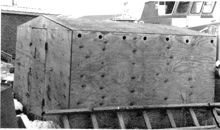
Small smokehouse made from plywood
