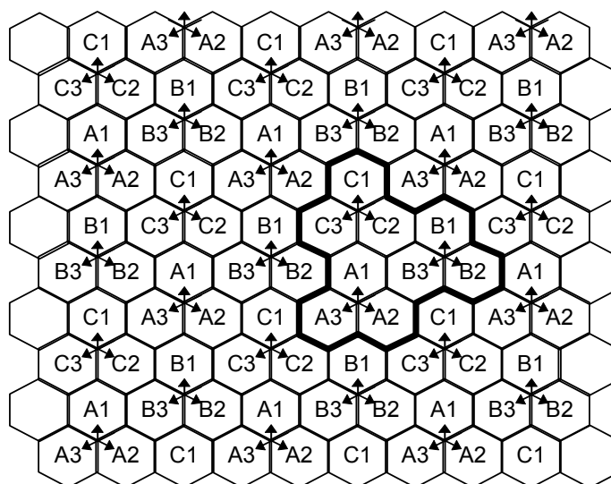
Figure 10-8 3/9 cell pattern
