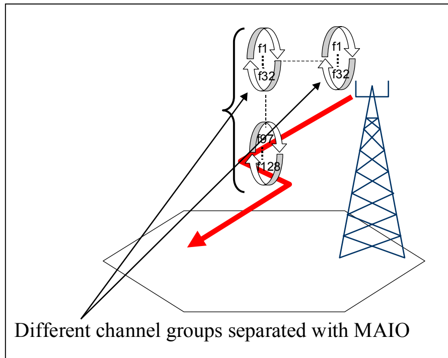
Figure 10-11. Re-use of Frequencies within a cell.
