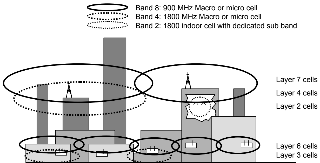
Figure 10-112 Hierarchical Cell Structures (HCS) divides the cell network into up to 8 layers
