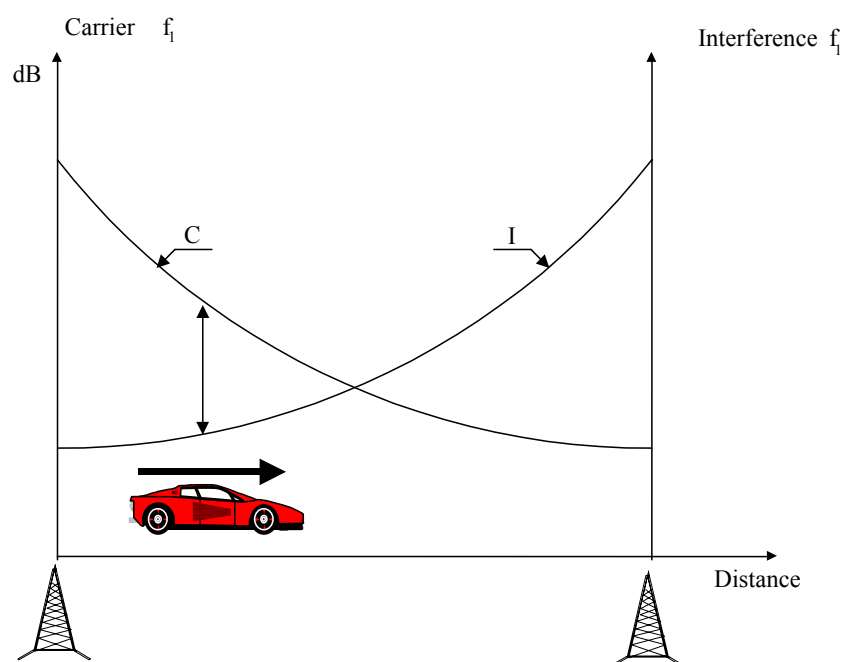
Figure 10-5 Co-channel interference
